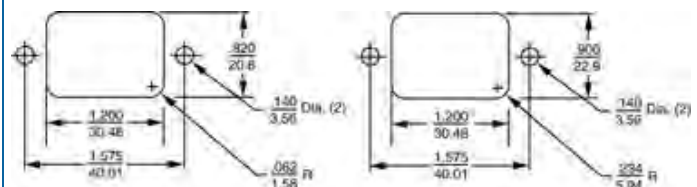
Panel cutout (Front mount)
