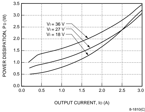
Figure 51. LC010F Typical Power Dissipation vs. Output Current at T_c = 25\text{ }^\circ\text{C}
