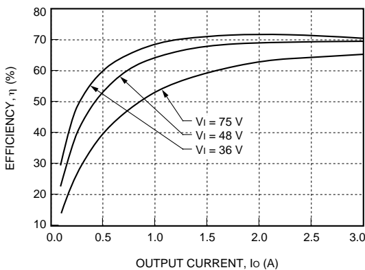
Figure 24. LW010D, 015D Typical Efficiency vs. Output Current at Tc = 25 °C
