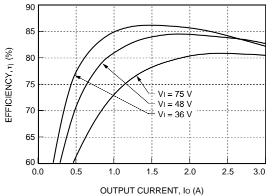
Figure 22. LW015A Typical Efficiency vs. Output Current at Tc = 25 °C
