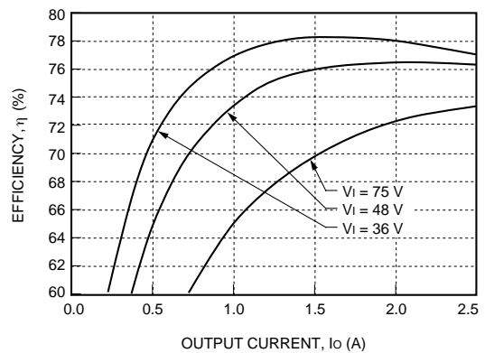
Figure 27. LW010F Typical Efficiency vs. Output Current at Tc = 25 °C
