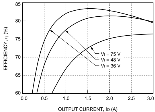
Figure 25. LW015F Typical Efficiency vs. Output Current at Tc = 25 °C
