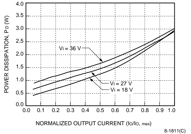
Figure 50. LC010A, B, C Typical Power Dissipation vs. Normalized Output Current at T_c = 25\text{ }^\circ\text{C}
