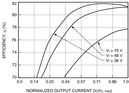
Figure 26. LW010A, B, C Typical Efficiency vs. Normalized Output Current at Tc = 25 °C
