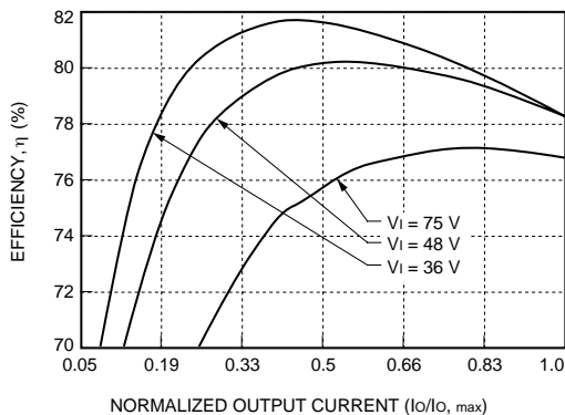
Figure 23. LW015B, C Typical Efficiency vs. Normalized Output Current at Tc = 25 °C
