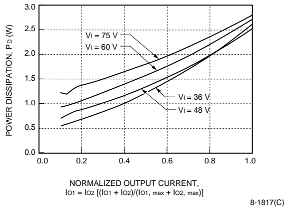
Figure 60. LW010AJ, BK, CL Typical Power Dissipation vs. Normalized Output Current at Tc = 25 °C
