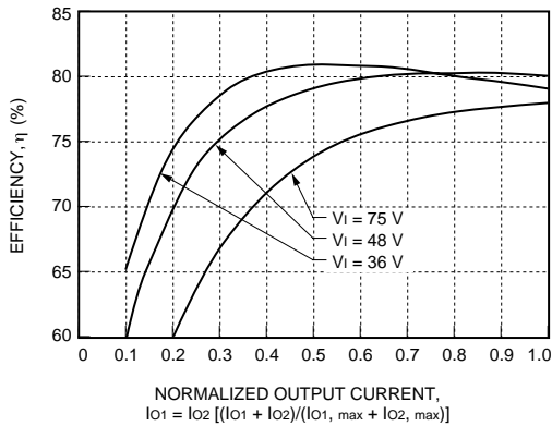
Figure 28. LW010AJ, BK, CL Typical Efficiency vs. Normalized Output Current at T c = 25 °C
