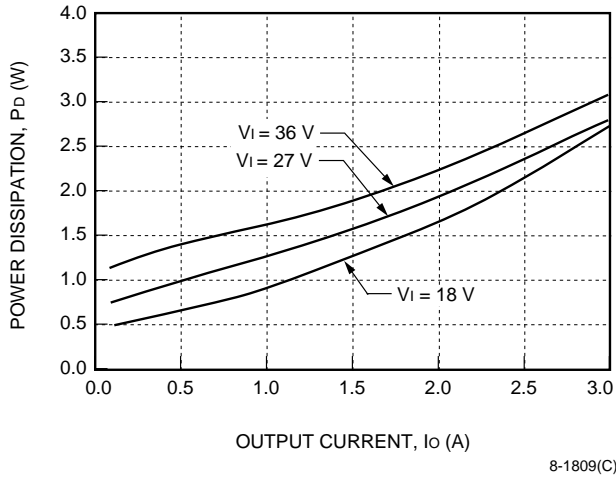
Figure 48. LC010D, 015D Typical Power Dissipation vs. Output Current at T_c = 25\text{ }^\circ\text{C}
