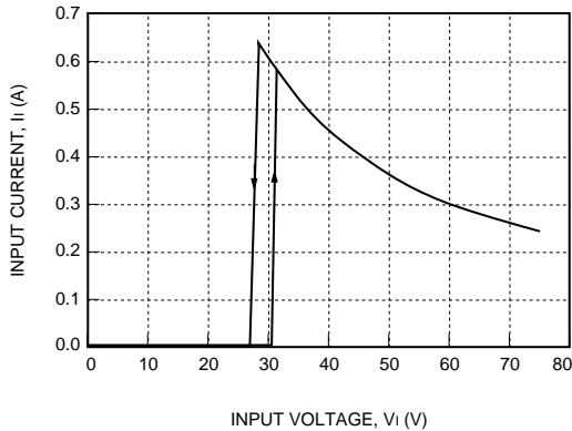
Figure 4. LW015 Input Current vs. Input Voltage at I_o = I_{o, max} and T_c = 25^\circ C
