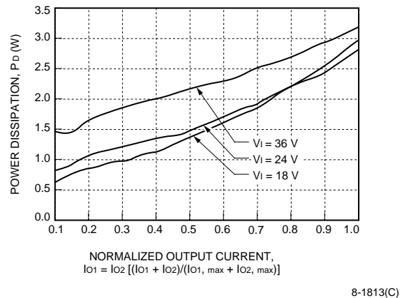
Figure 52. LC010AJ, BK, CL Typical Power Dissipation vs. Normalized Output Current at T_c = 25\text{ }^\circ\text{C}
