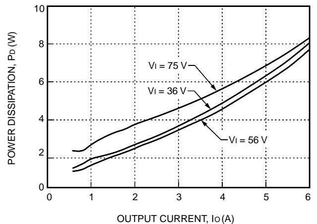
Figure 13. LW030A Power Dissipation vs. Output Current
