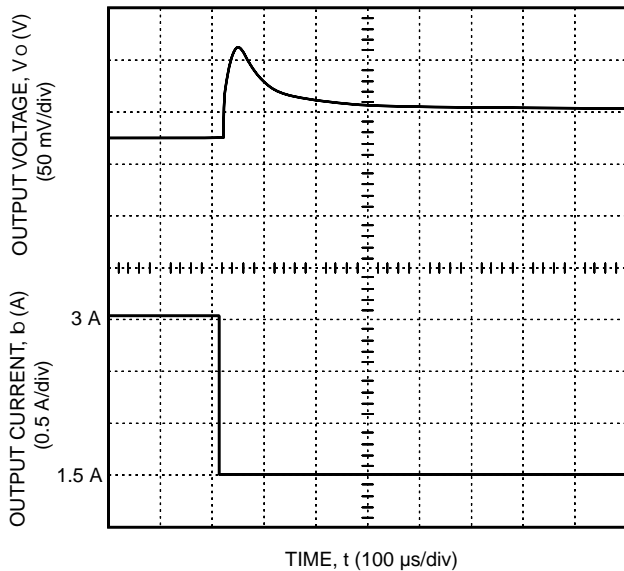
Figure 5. Typical Output Voltage for a Step Load Change from 50% to 25%
