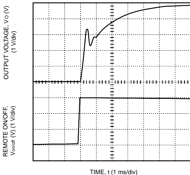
Figure 6. Typical Output Voltage Start-Up when Signal Applied to Remote On/Off
