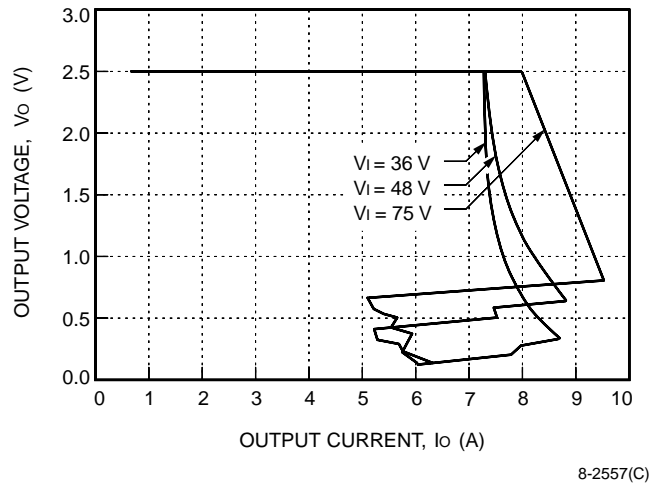
Figure 4. JW030G-M Typical Output Characteristics
